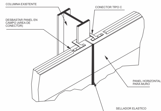
ISOMETRIA
