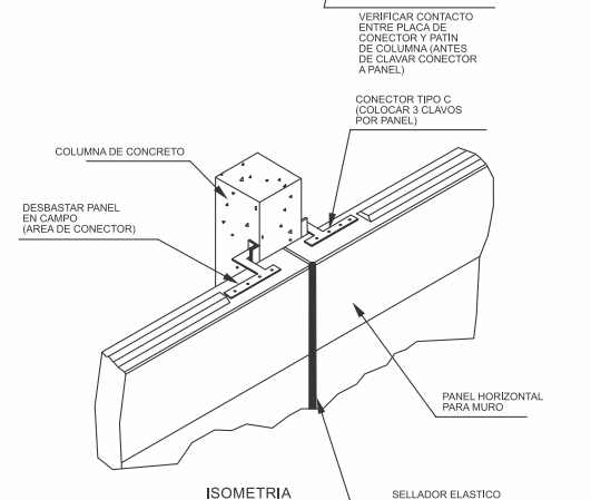
ISOMETRIA
